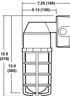
Wall Fluorescent/HID
