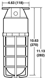
Ceiling Fluorescent/HID
