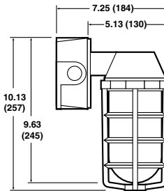
Wall Incandescent
