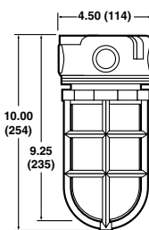
Ceiling Incandescent
