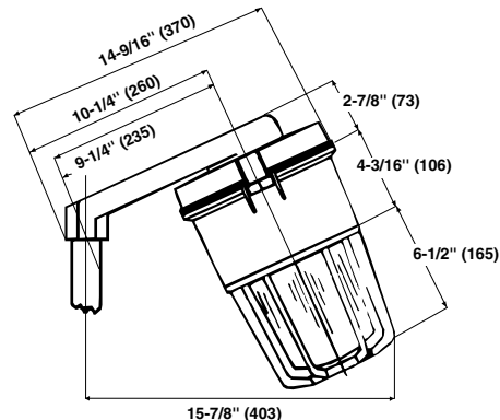
90° STANCHION MOUNT
