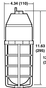
Pendant Fluorescent/HID
