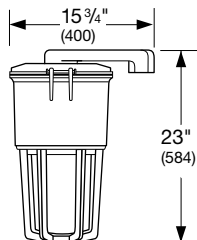
Straight Stanchion
