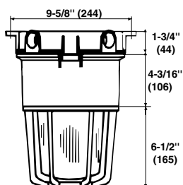
CEILING MOUNT
