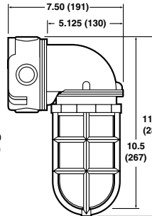
Wall Incandescent
